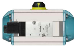
Solenoid valve
