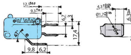
W3 for 6.35 mm clips (6.3 x 0.8)
