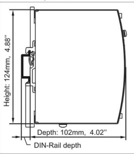
Fig. 19-2 Side view
