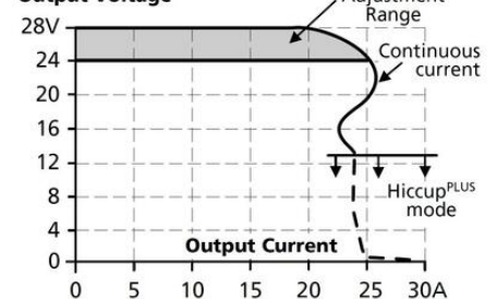
Output Voltage
