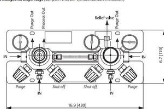
KPA – Automatic changeover, single-stage (Compact Panel, 2x1 cylinder standard manometer)
