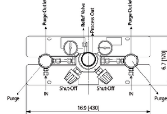
KPME - Manual changeover (for 2x1 cylinder, manual changeover, with relief valve)
