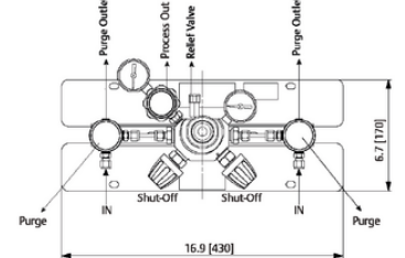
KPME2 - Manual changeover (Compact Panel, 2x1 cylinder, manual changeover with relief valve dual stage)
