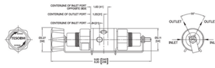
CR441800 SERIES CHANGEOVER SYSTEMS (HIGH PRESSURE)
