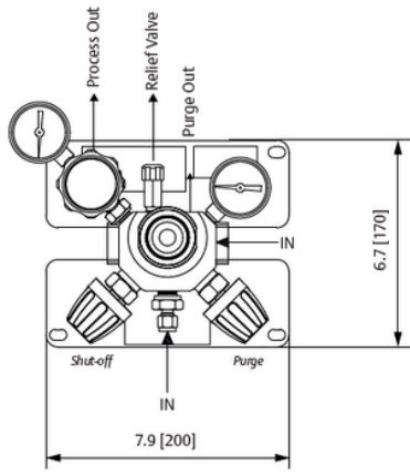
KP12 (Compact panel, 1 cylinder, dual stage)
