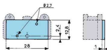
Y (on request) side plate
