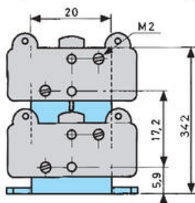
K2 (on request) 2-pole vertical mounting plate
