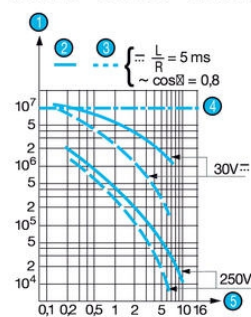
Operating curve for type 83 132 0 - 83 133 0 - 83 134 0
