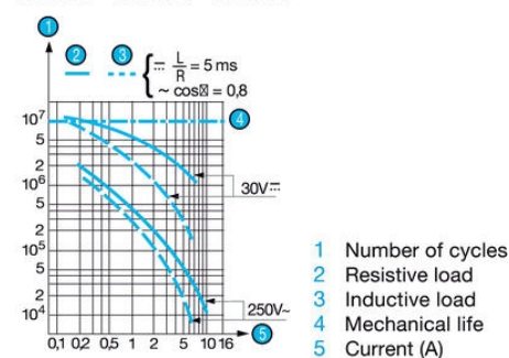
Operating curve for type 83 132 0 - 83 133 0 - 83 134 0
