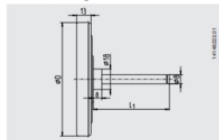
Smooth connection, with 18 mm collar diameter for thermowell mounting
