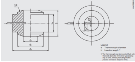
Model TC90-C, high-pressure thermocouple with lens-type sealing ring or sealing cone
