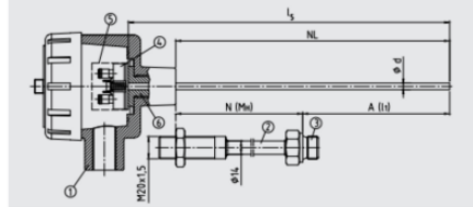
Neck tube with counter nut to head
