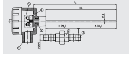
"Nipple-union-nipple" neck tube
