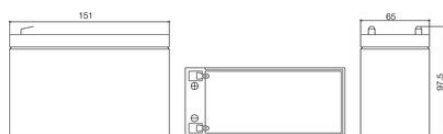
Faston flat connector 4,8 mm
