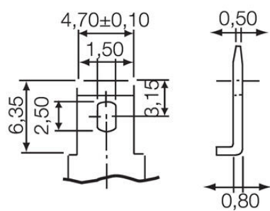
Faston flat connector 4,8 mm
