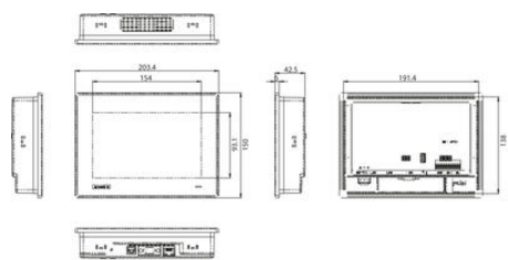
Panel Cut Out Dimensions: 192 x 138.5 mm (7.56" x 5.45")
