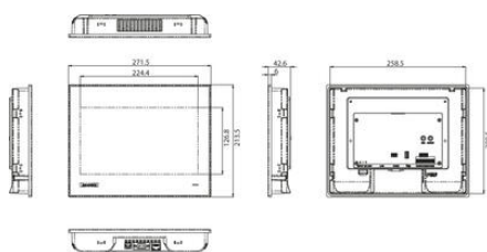
Panel Cut-out Dimensions: 260 x 201.5 mm (10.24" x 7.93")
