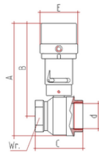
OVERALL DIMENSIONS DOUBLE ACTING
