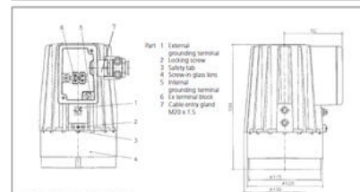
Variant 2 (incl. terminal box Ex d)
