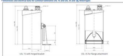
* Dimensions and electrical data for Lumistar luminaires USL 15 and USL 35 and tested types
