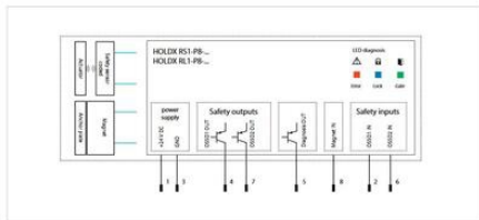
HOLDX R_1 standalone B-pin pigtail without EDM function
