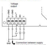
Pin assignment of series LK, LW, LI
