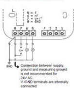
Pin assignment of series LK, LW, LI
